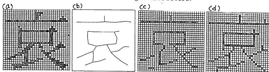
Fig.6 Examples of distorted patterns and skeleton patterns for Japanese Kanji characters.
