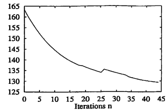
Fig.2 Example of learning curve.
